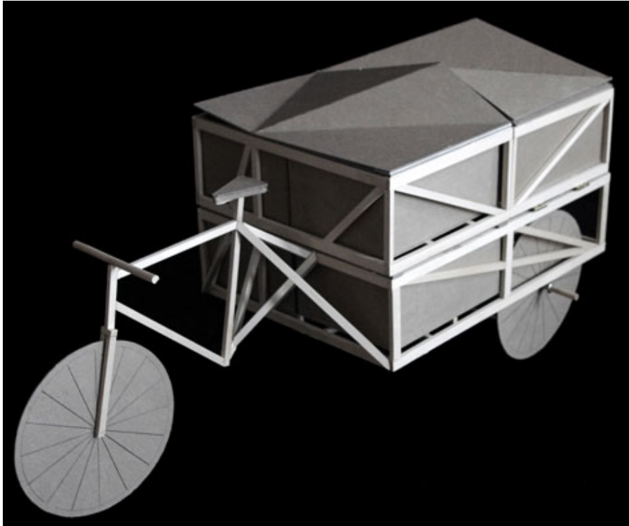
Bike integrated into cart
