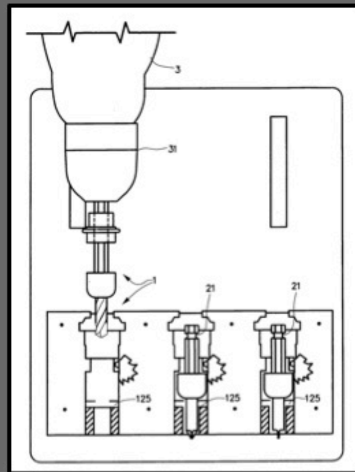
Drill and driver bit dispensing system US 7275659 B2
