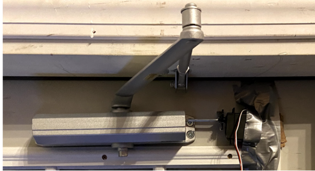
Speed Adjustment & Modified Door Closer
